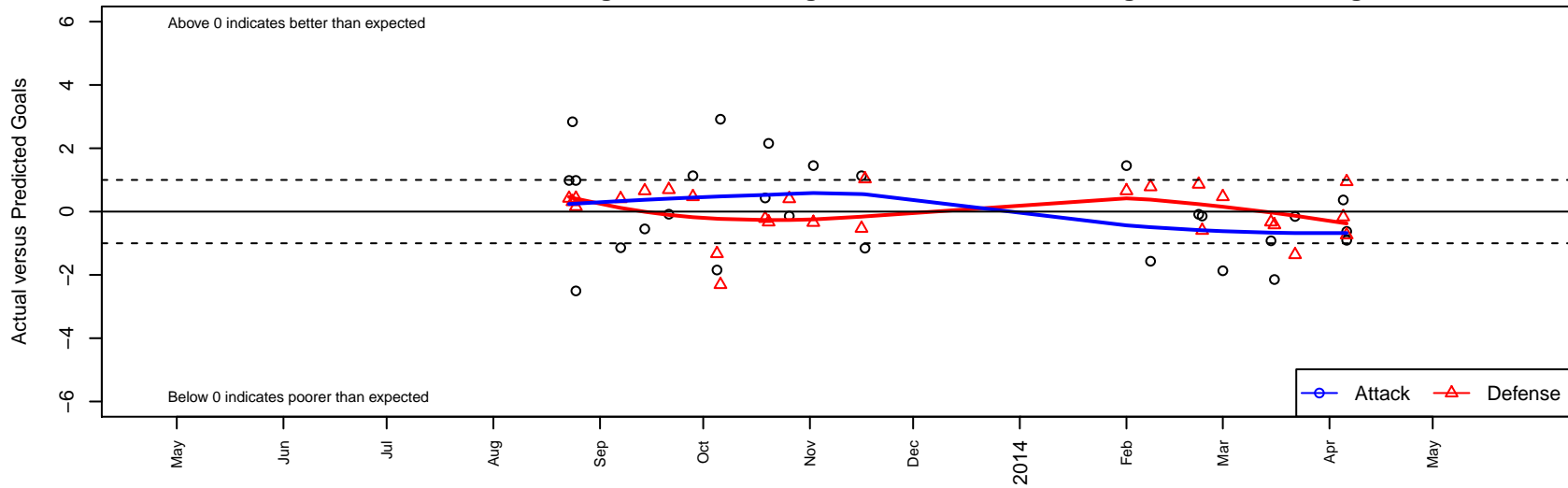
Cascade FC Green G01 Dots are actual minus expected GF (blue circles) and GA (red triangles). Blue line is smoothed change in attack strength. Red is smoothed change in defense strength.
